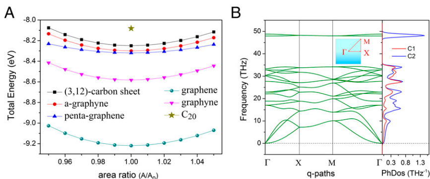
Fig. 2. (A) Area dependence of total energy per atom for some 2D carbon allotropes. The total energy of the experimentally identified dodecahedral \text{C}_{20} cage is also calculated and plotted here for comparison. (B) Phonon band structures and PhDOS of penta-graphene. (Inset) High-symmetric q -point paths: \Gamma (0, 0) \rightarrow X (1/2, 0) \rightarrow M (1/2, 1/2) \rightarrow \Gamma (0, 0) .
